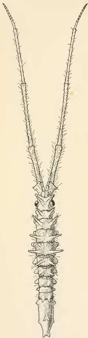
FIG. 27.—ARCTURUS DIVERSISPINIS. \times 1.2. FEMALE. (Drawn by Miss V. Dandridge.)
